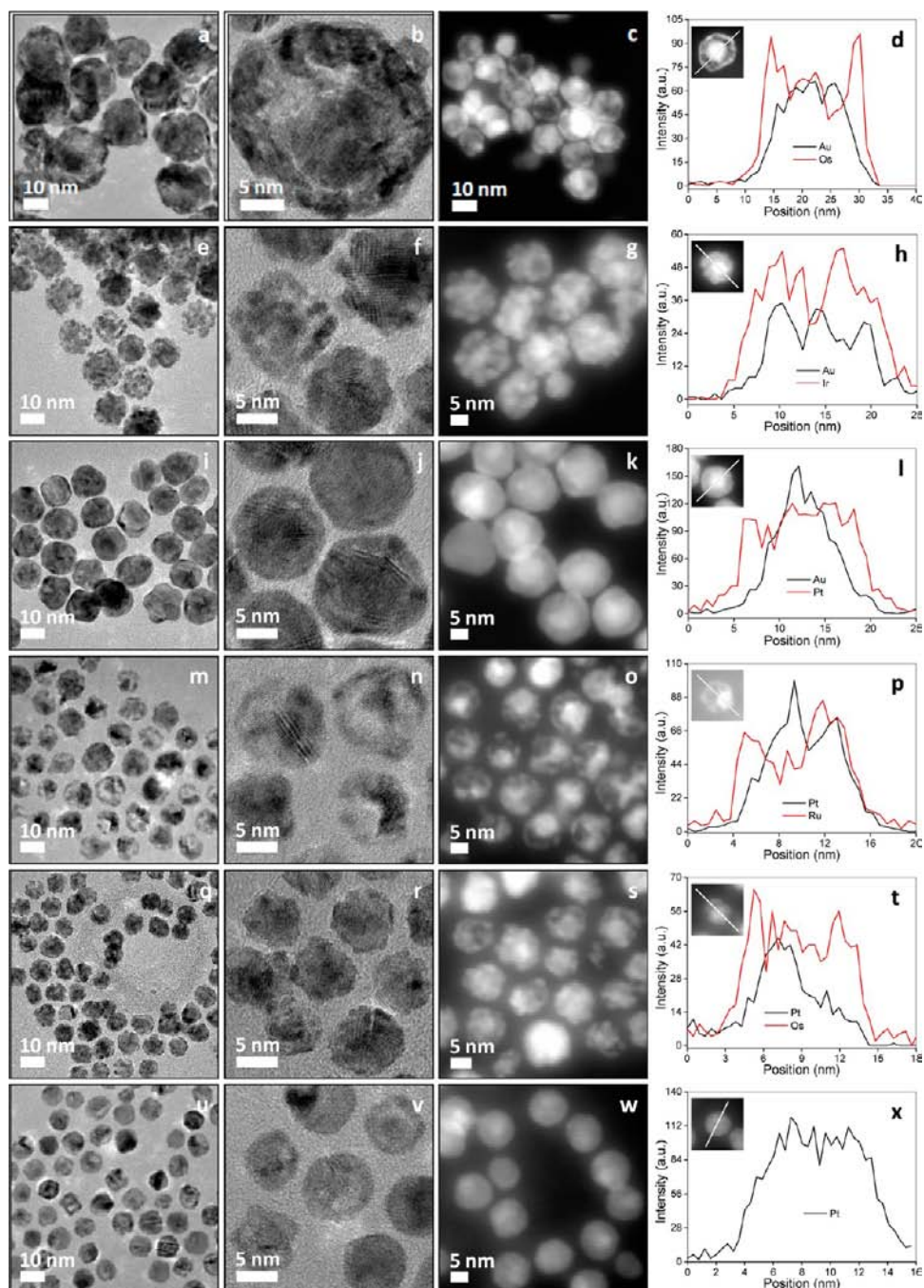
Figure 4. Cage-bell structured (CBS) metal nanoparticles: (a, e, i, m, q, and u) TEM images, (b, f, j, n, r, and v) HRTEM images, (c, g, k, o, s, and w) STEM images, and (d, h, l, p, t, and x) element profiles of (a–d) CBS Au–Os, (e–h) CBS Au–Ir, (i–l) CBS Au–Pt, (m–p) CBS Pt–Ru, (q–t) CBS Pt–Os, and (u–x) CBS Pt–Pt nanoparticles.
